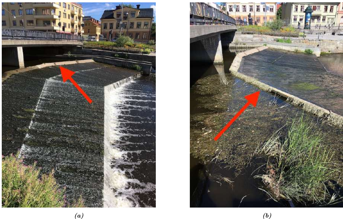
Figure 9: Photographs of Islandsfallet a) looking upstream and b) looking downstream. The extra threshold added to Islandsfallet in summer is marked by the red arrow. (Photo: Roger Herbert)
