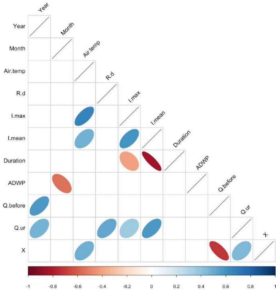
Figure 18: The significant correlations for the parameters, indicated in color. A red colour signals negative correlation and a blue colour positive correlation. The ellipse symbol is shaped narrower the stronger the correlation is and it is tilted in the direction of the correlation. The confidence level is 95%. Empty squares indicate parameters did not show significant correlations.
