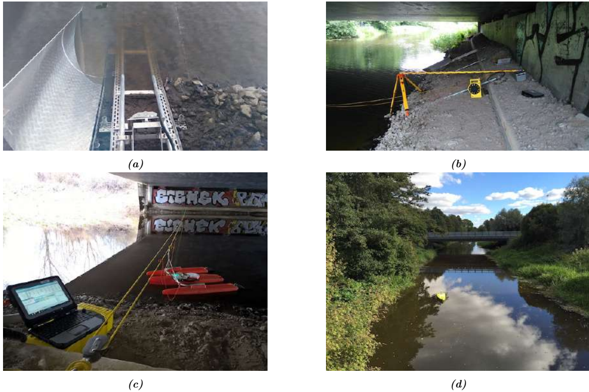
Figure 10: Photos of the index station at Bärbyleden. a) The hydroacoustic velocity meter submerged. b) Adjusting the cross-section area. c) Controlling index station with ADCP boat. d) Looking downstream towards the index station. (Photo: Mikael Lennermark)
