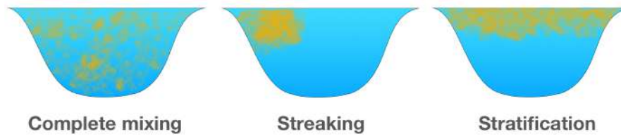
Figure 4: Illustration of how complete mixing, streaking or stratification affect the concentration in a river. The yellow colour illustrates the concentration of pollutants. The figure shows a river in cross section.
