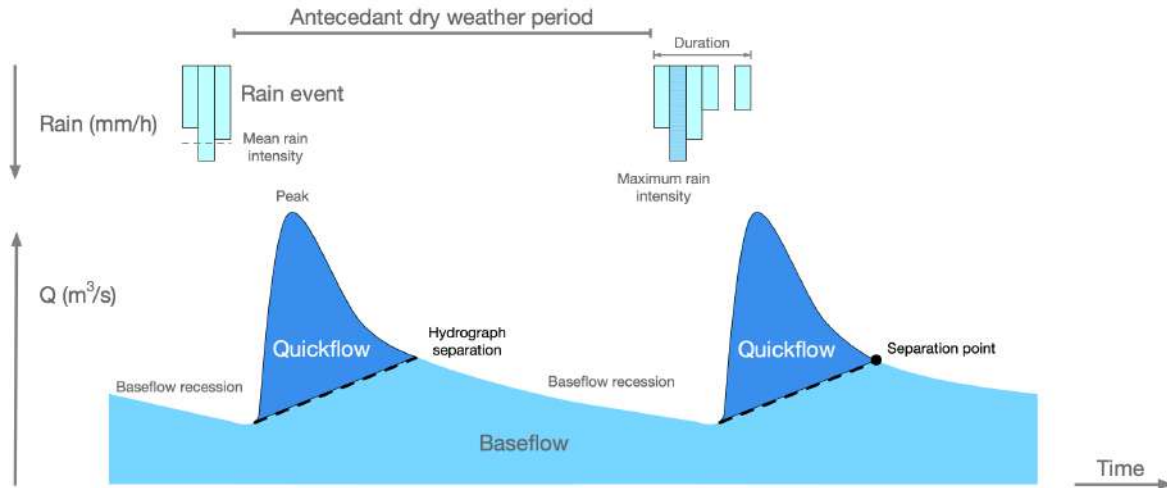
Figure 2: A hydrograph, flow ( Q ) against time, with a hyetograph, rain intensity against time, above. Quickflow in dark blue and baseflow in light blue with a dotted line representing the hydrograph separation.
