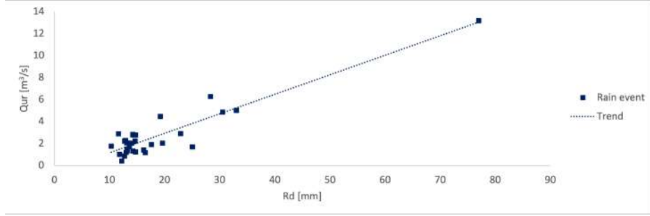
Figure 23: Q_{ur} as a function of R_d . The dotted line shows a linear regression with the equation y = 0.18x - 0.62 , n = 31 , R^2 = 0.86 , p = 9e^{-14} .
