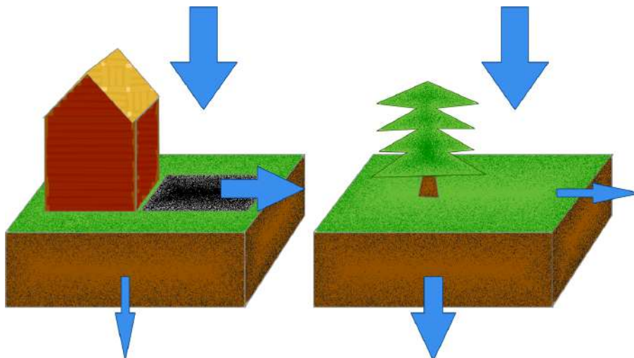
Figure 1: Simplified illustration of urban hydrology compared to natural hydrology. Impervious surfaces such as roofs and roads (left) create more surface runoff (right arrow) and less infiltration (downwards arrow below ground) than more permeable natural surfaces (right).
