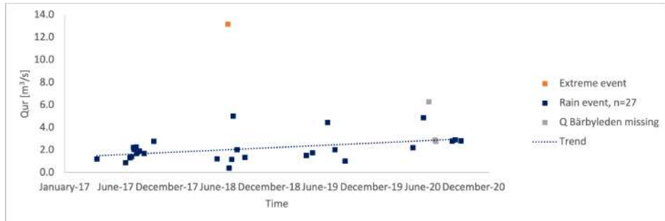
Figure 24: The urban runoff quickflow Q_{ur} as a function of time. The dotted line shows a linear regression with slope +0.44 \text{ m}^3/\text{s}/\text{year} , n = 27 , R^2 = 0.18 .
