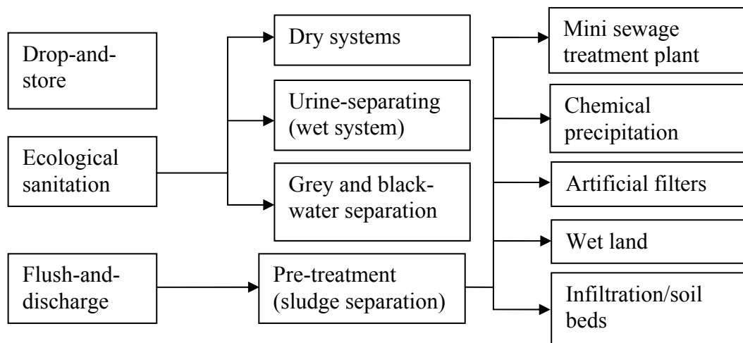
Figure 6 Small-scale solutions for sewage treatment (modified from Palm et al. 2003).
