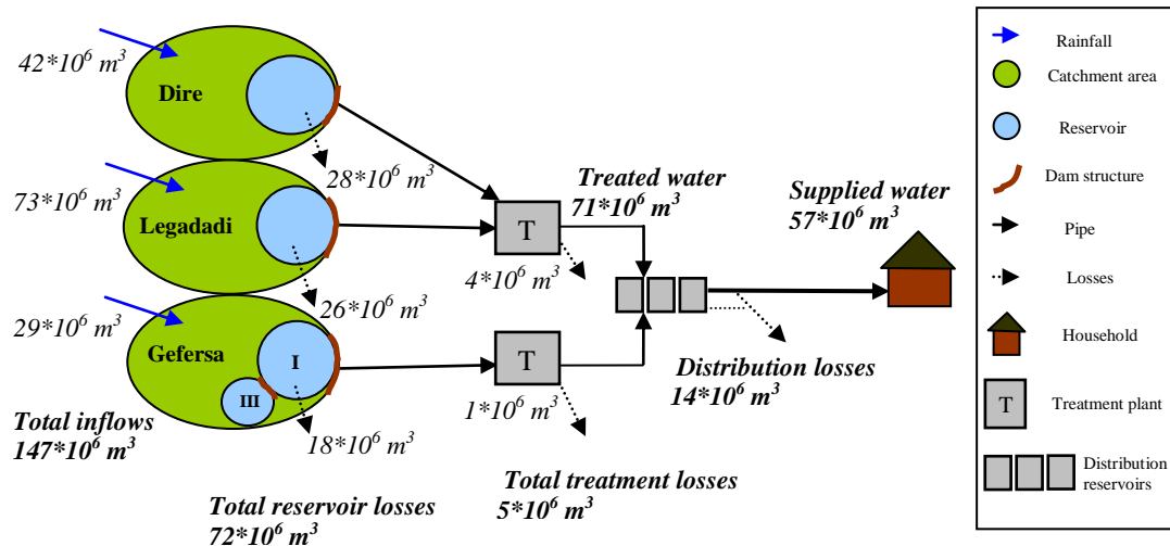
Figure 23. Flow chart used for describing annual flows in the studied water supply system.
