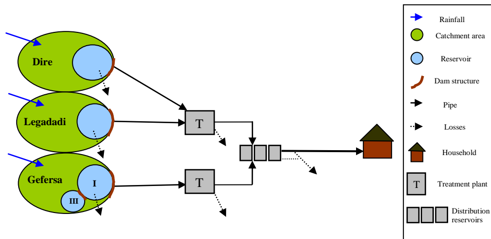
Figure 13. The flow chart graphics used for describing the water supply system. All the flows (arrows) were quantified.
